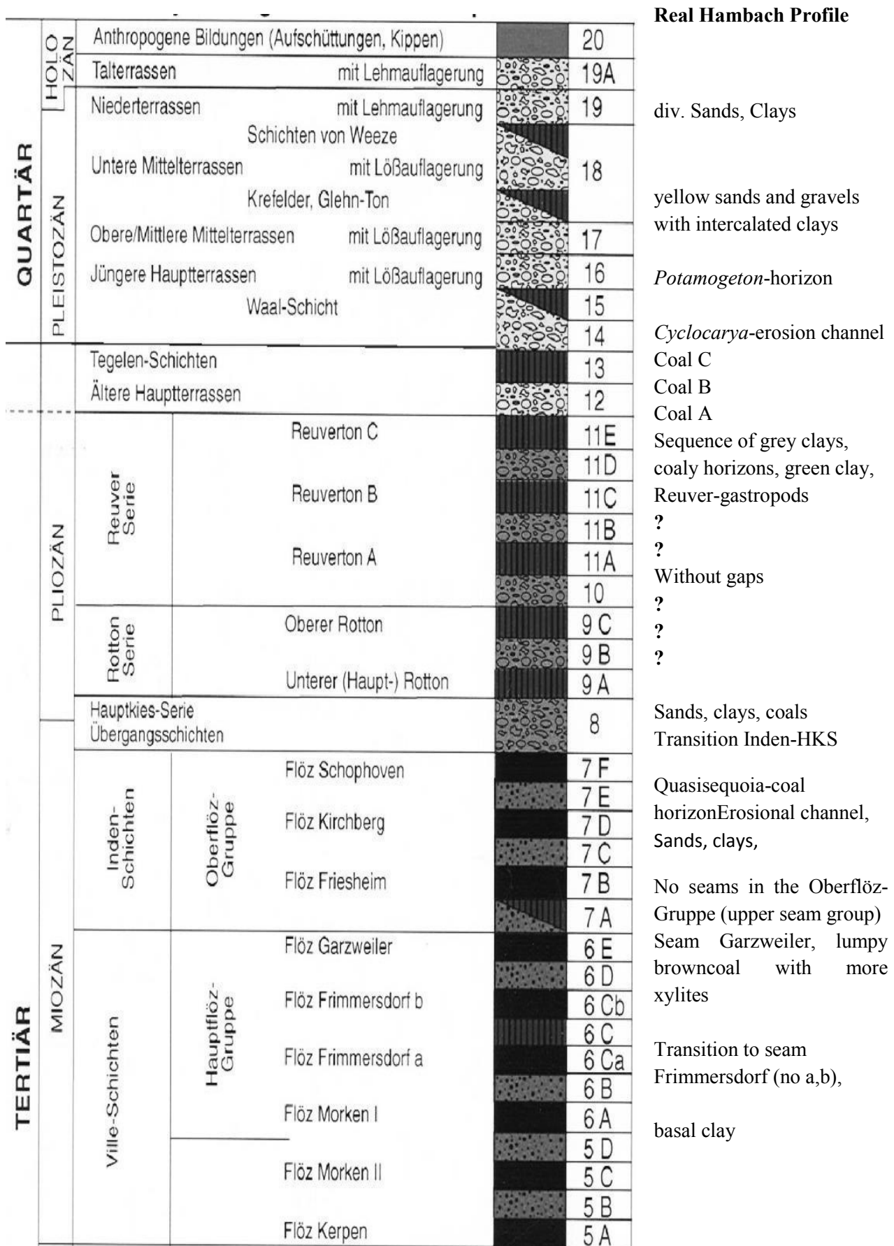
Text-fig. 4: Ideal profile after SCHNEIDER & THIELE 1965 in the opencast coal mines of the RWE and to the right with special names and remarks of the layers in opencast mine Hambach
